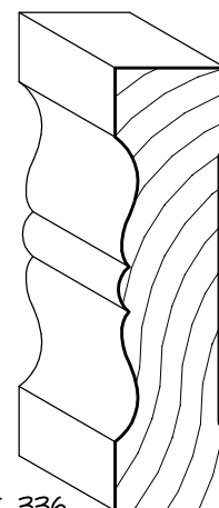
SMC-336 1" x 4" COAST GUARD CASING
