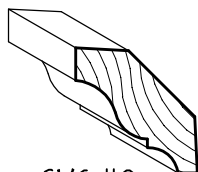
SMC-110 \frac{3}{4} " x 2\frac{1}{4} " CROWN
