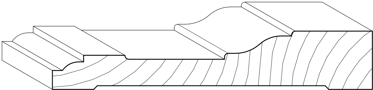
SMC-358 1" x 5 1/2" CASING
