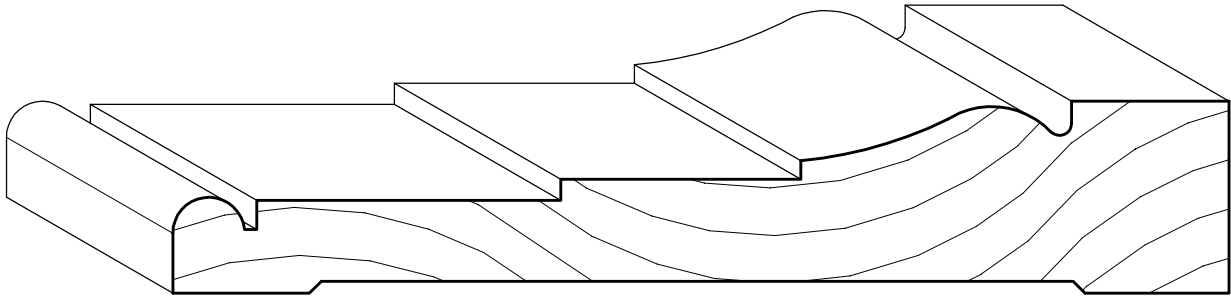
SMC-357 1" x 5 1/2" CASING
