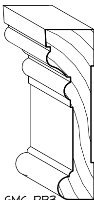
SMC-RB3 1" x 3 1/2" CASING
