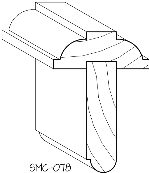
1 5/8" x DOOR THICKNESS T-ASTRAGAL
