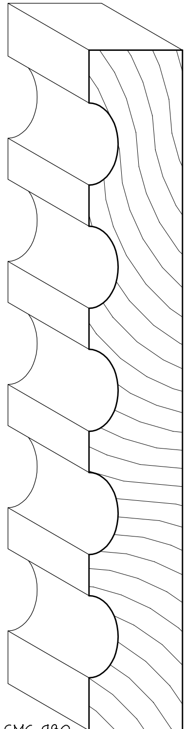
SMC-980 1" x 1 1/4" FLUTED PILASTER
