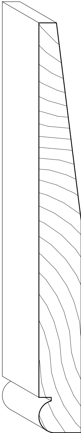
BEADED BEVEL SIDING
