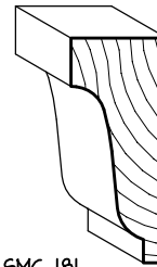
SMC-181 1 1/2" x 3 1/2" RAKE MOULD
