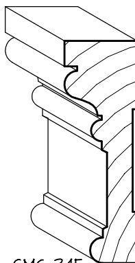
SMC-345 1" x 3 1/4" CASING
