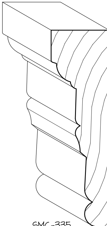
SMC-335 1" x 3 1/2" FRANKLIN CASING
