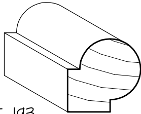
SMC-193 3/4" CORNER BEAD
