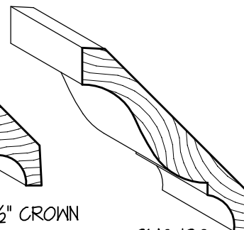
SMC-120 \frac{3}{4} " x 4\frac{1}{2} " CROWN
