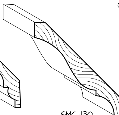
SMC-130 \frac{3}{4} " x 5\frac{1}{4} " CROWN MOULD
