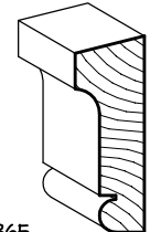
SMC-365 1 1/8" x 3" EXTERIOR WINDOW SILL APRON
