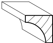
SMC-121 \frac{1}{2}'' \times \frac{1}{2}'' COVE MOULD
