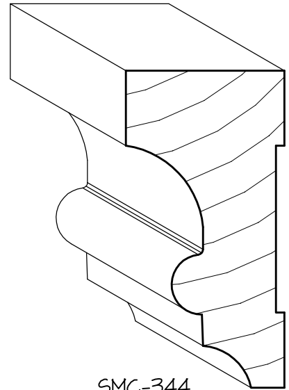
SMC-344 1 1/4" x 2 3/8" CASING
