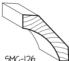
SMC-126 \frac{3}{4} " x 2\frac{3}{4} " COVE MOULD
