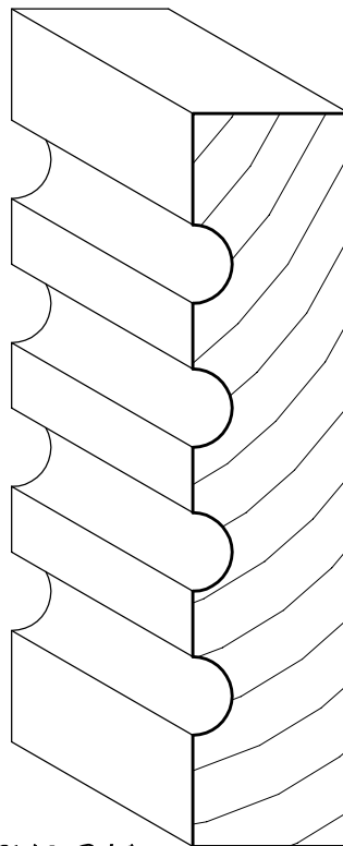
SMC-349 3/4" x 3 1/2" FLUTED CASING
