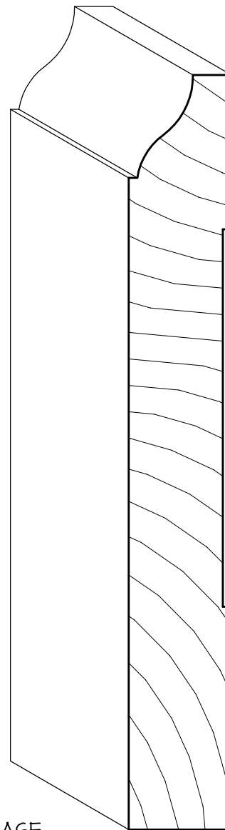
OG BASE SMC-818 \frac{3}{4} " x 3\frac{1}{2} " SMC-819 \frac{3}{4} " x 4\frac{1}{2} " SMC-820 \frac{3}{4} " x 5\frac{1}{2} " SMC-821 \frac{3}{4} " x 7\frac{1}{4} "
