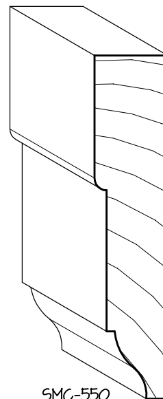
SMC-550 3/4" x 3 1/2" APRON
