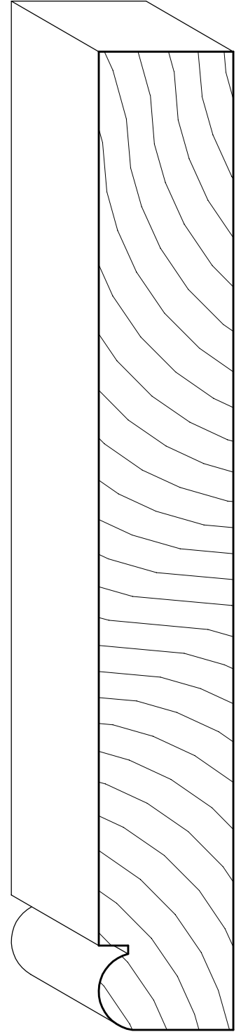
BEADED 1 EDGE SMC-496 1'' \times 3\frac{1}{2}'' SMC-497 1'' \times 5\frac{1}{2}'' SMC-498 1'' \times 7\frac{1}{4}'' SMC-499 1'' \times 9\frac{1}{4}''
