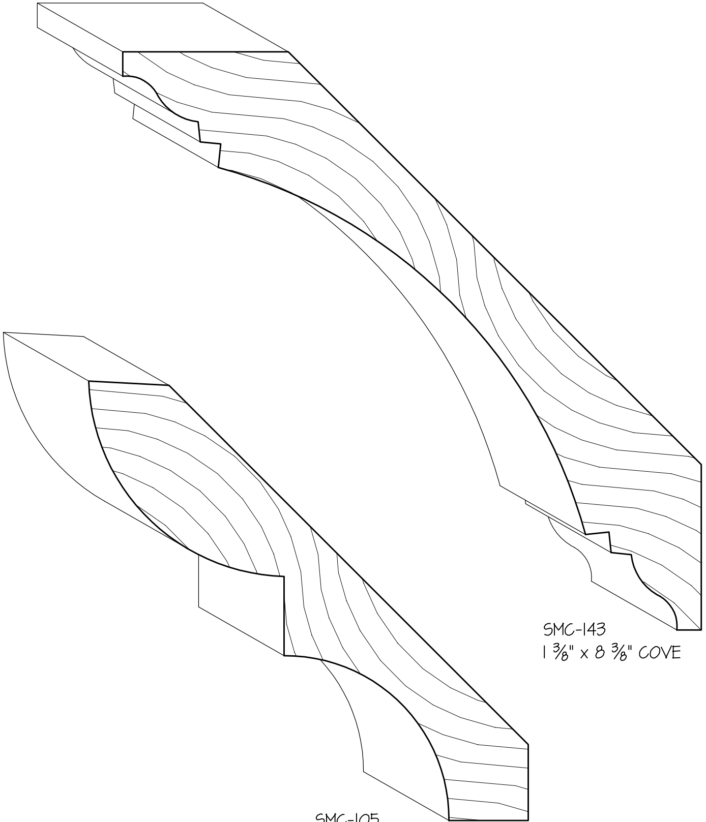
SMC-105 1 1/8" x 6 3/8" BED
