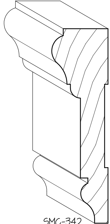
SMC-342 1" x 3 1/2" CASING
