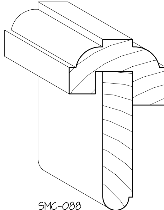
1 5/8" x DOOR THICKNESS KERFED ASTRAGAL
