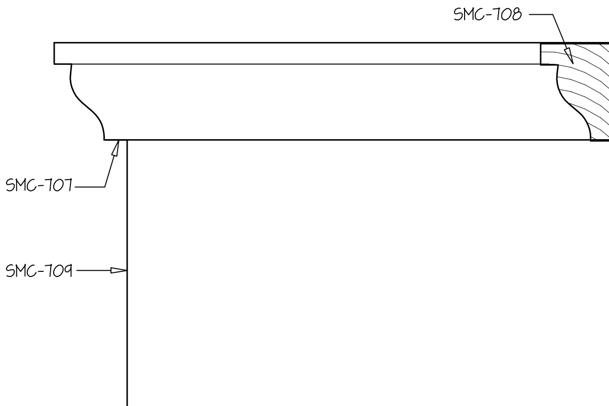
SMC-709 SQUARE MODILLION BLOCK, 2\frac{3}{4} " x 3\frac{1}{2} " x 5" SMC-707 MODILLION PLATE, 1" x 4\frac{1}{2} " x 5\frac{1}{2} " SMC-708 MODILLION MOULDING, \frac{3}{4} " x 1"
