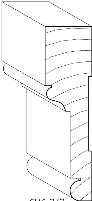
SMC-343 1" x 3 1/2" CASING
