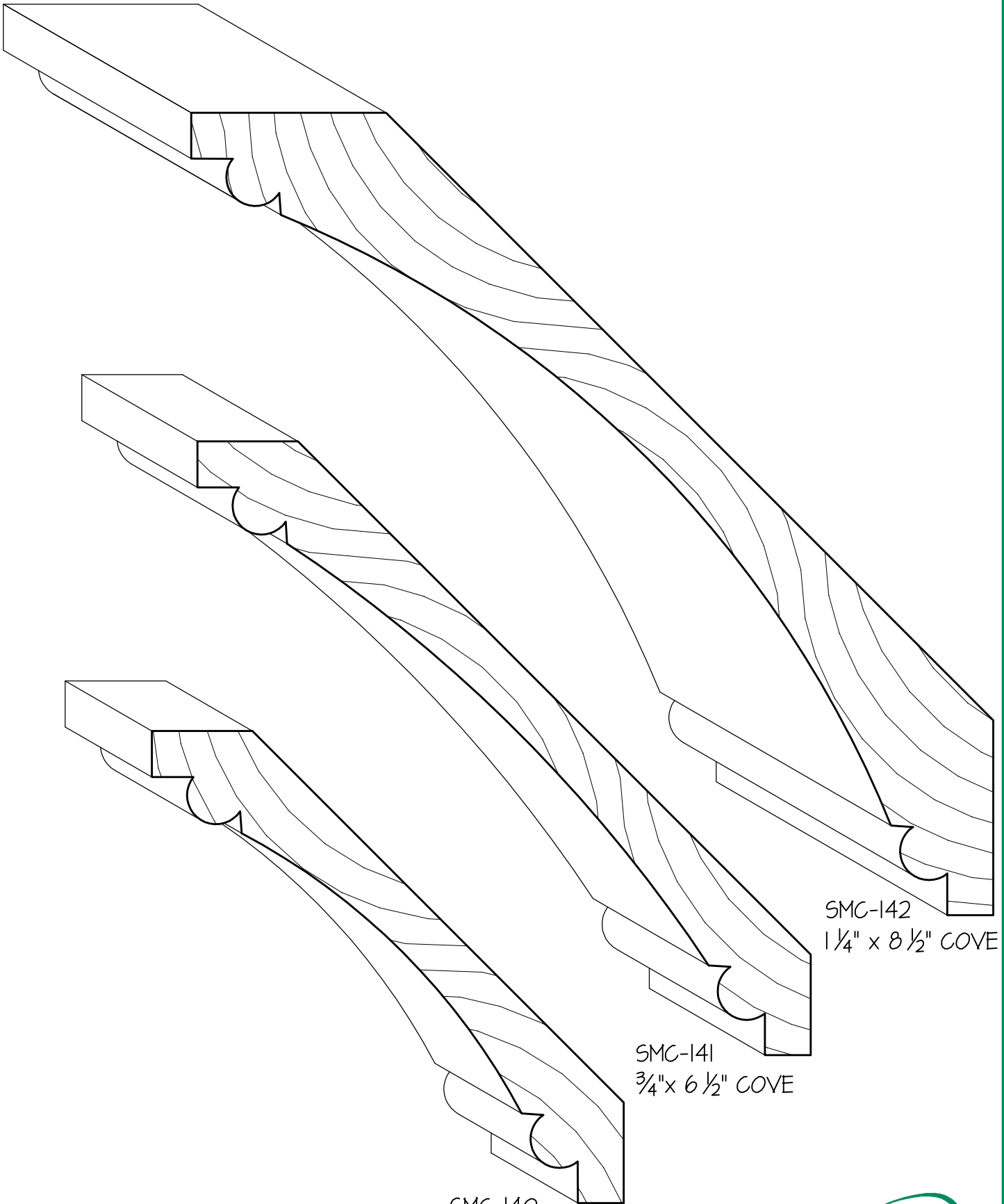
SMC-140 3/4" x 5" COVE
