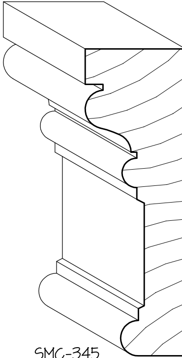
SMC-345 1" x 3 1/4" CASING
