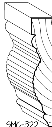
SMC-322 3/4" x 3 1/2" REEDED CASING
