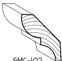
SMC-102 \frac{3}{4} " x 2\frac{3}{4} " BED MOULD
