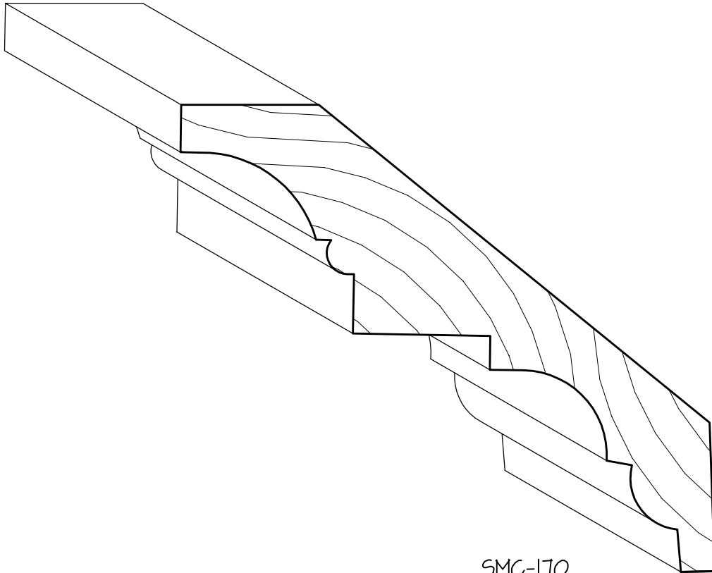
SMC-170 1 1/8" x 5 1/4" CURTIS CROWN
