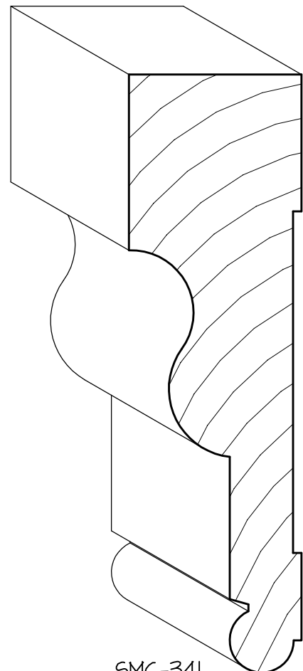
SMC-341 1/4" x 4 3/8" CASING
