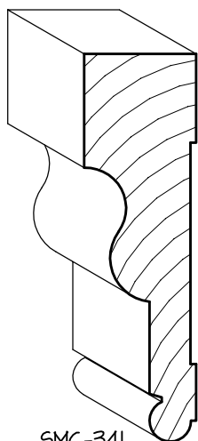
SMC-341 1 1/4" x 4 3/8" CASING
