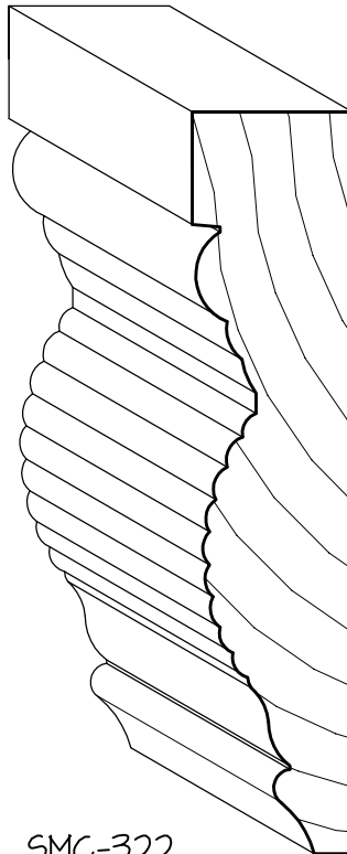
SMC-322 \frac{3}{4} " x 3\frac{1}{2} " REEDED CASING
