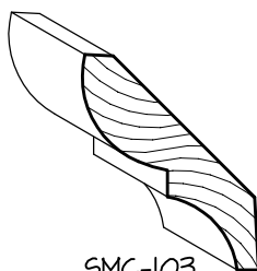
SMC-103 \frac{3}{4} " x 3\frac{1}{4} " BED MOULD
