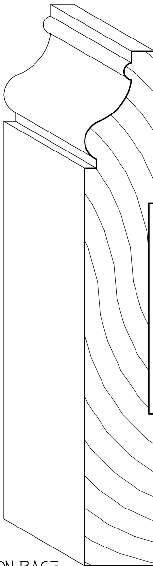
BENTON BASE SMC-830 \frac{3}{4} " x 5\frac{1}{2} " SMC-831 \frac{3}{4} " x 7\frac{1}{4} "
