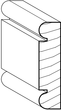
SMC-470 BEADED MULL TRIM
