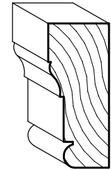
SMC-370 1 1/2" x 3 1/2" BRICK MOULD
